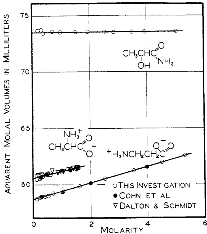
FIG. 4. The apparent molal volumes of \alpha -alanine, \beta -alanine, and lactamide at 25°C.
