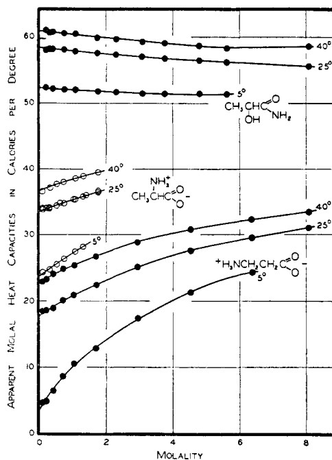
FIG. 3. The apparent molal heat capacities of \alpha -alanine, \beta -alanine, and lactamide at 5°, 25°, and 40°C.
